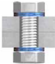
Through holes require two pairs of SUR-LOCK washers.
