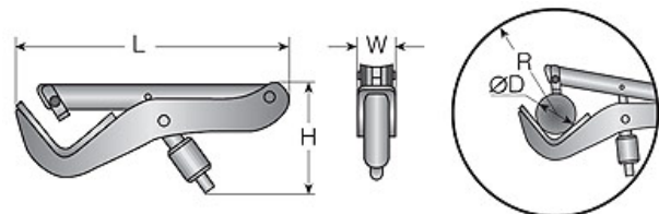
NES 3 EXTERNAL TOOL IBS No. 99163
