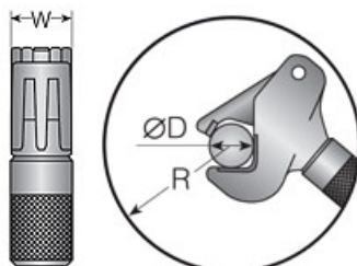
NES 1 EXTERNAL TOOL IBS No. 99152
