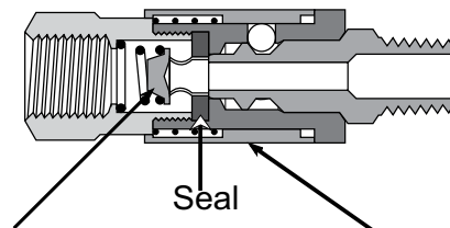
CONNECTED
