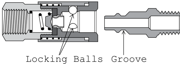
COUPLER
