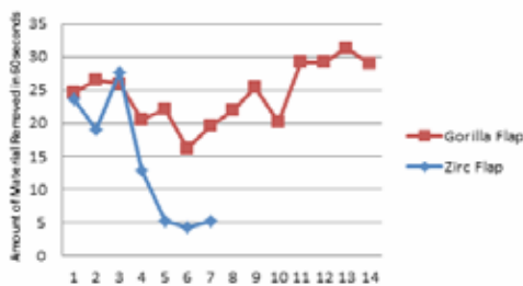
Removal Rate on Stainless Steel
