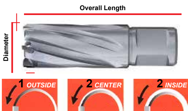
Triple Edge Cutters — Superior ultra-hard tungsten carbide tips, balanced in three different positions permit higher feed rates and increased hole making in structural steel and steel plate.
